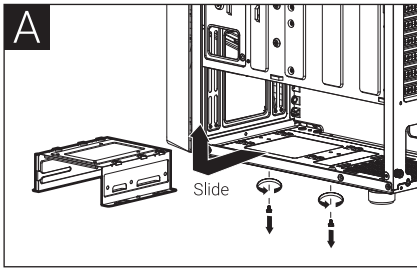
(5a) Install 2.5" SSD x 1
