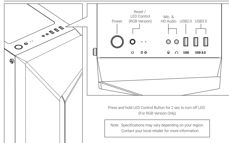
I/O Panel
