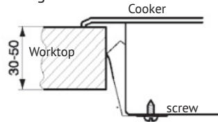
installation sheet
