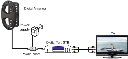
Installation 1: directly connected to HDTV connected through digital converter box (Fig.4)
