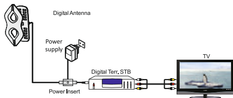
Installation 1 : directly connected to HDTV Connected through digital converter box (Fig.4)
