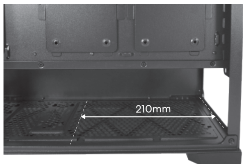
PSU Length
