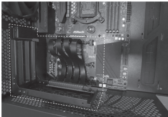
LANCOOL II - 1X Vertical GPU kit
