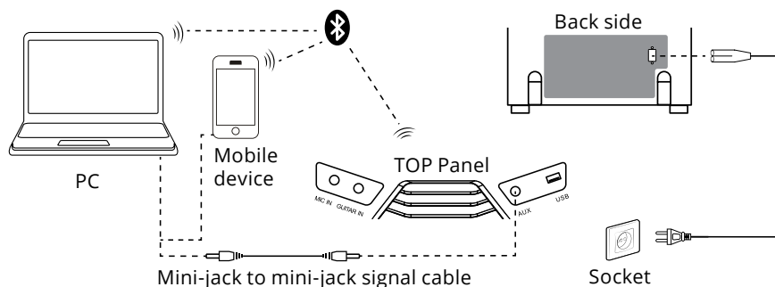
Fig.2. Connection diagram
