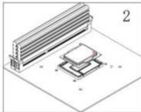
2. INSTALL CPU IN SOCKET FOLLOWING TRIANGLE SIGN
