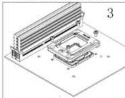
3. INSTALL BCF WITH ORIGINAL ILM SCREWS
